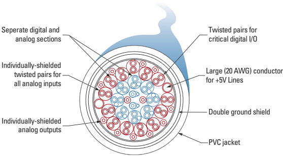
Figure 1. SH68-68-EP Cable
