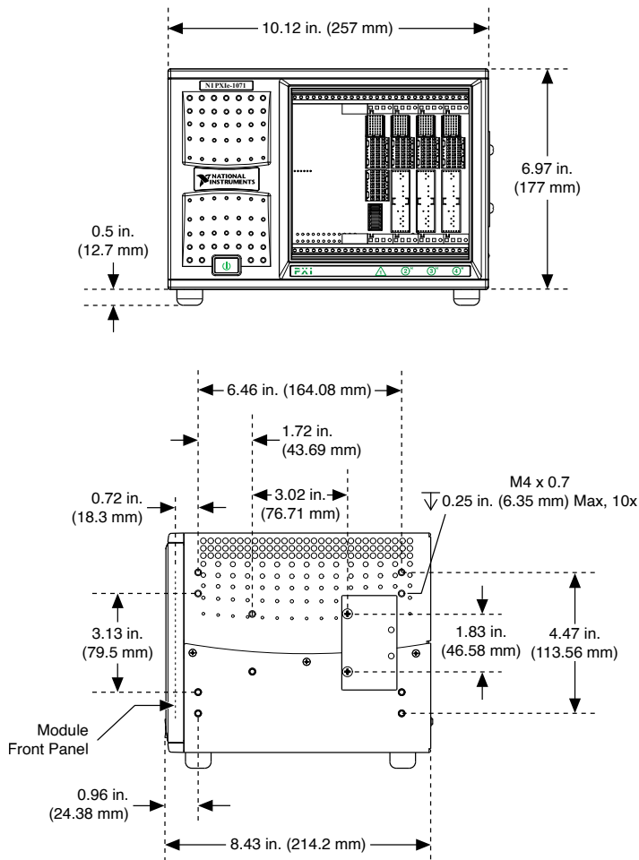
Figure 1. PXle-1071 Chassis Dimensions (Front and Side)
