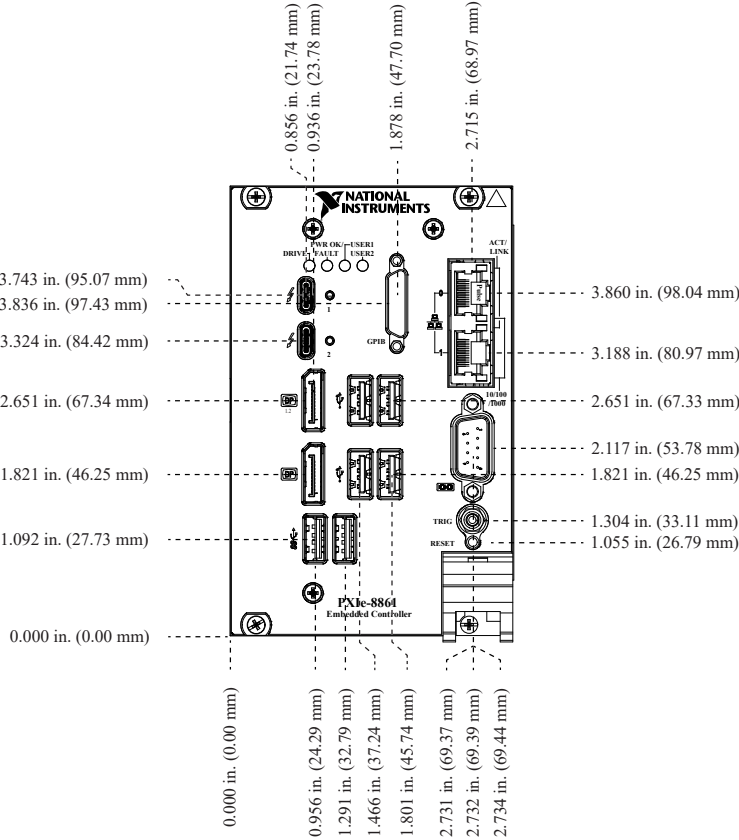
Figure 2. PXle-8861 Front Panel Layout and Dimensions
