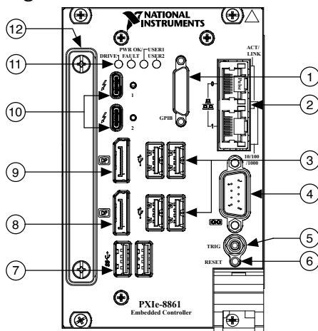
Figure 1. PXIe-8861 Front Panel
