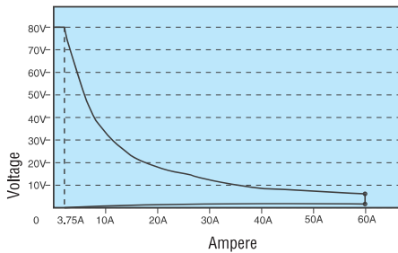
MODEL 63103 INPUT CHARACTERISTICS
