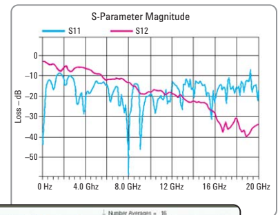
The DCA_J, TDR module and S-parameter software covers the challenge of characterizing complex circuitry such as backplanes.
