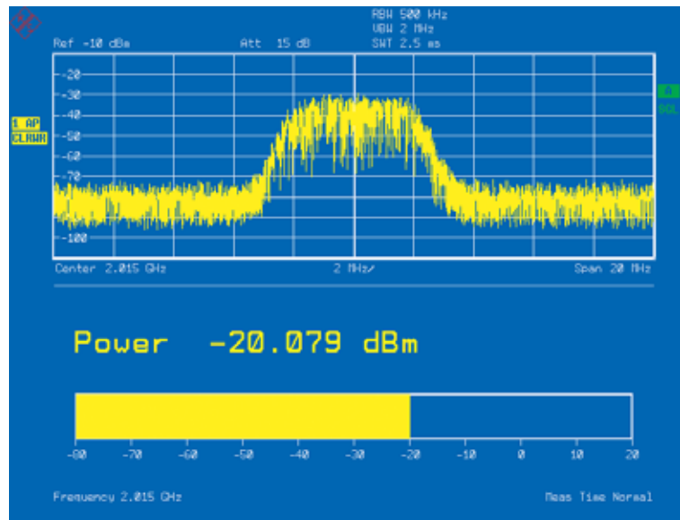
Power measurement of a 3GPP HSDPA signal.
