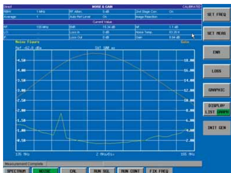
Noise figure measurement with the option R&S®FS-K30.
