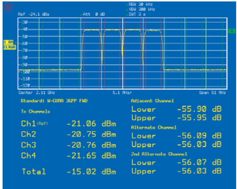
ACP measurement on a WCDMA signal with 4 channels.
