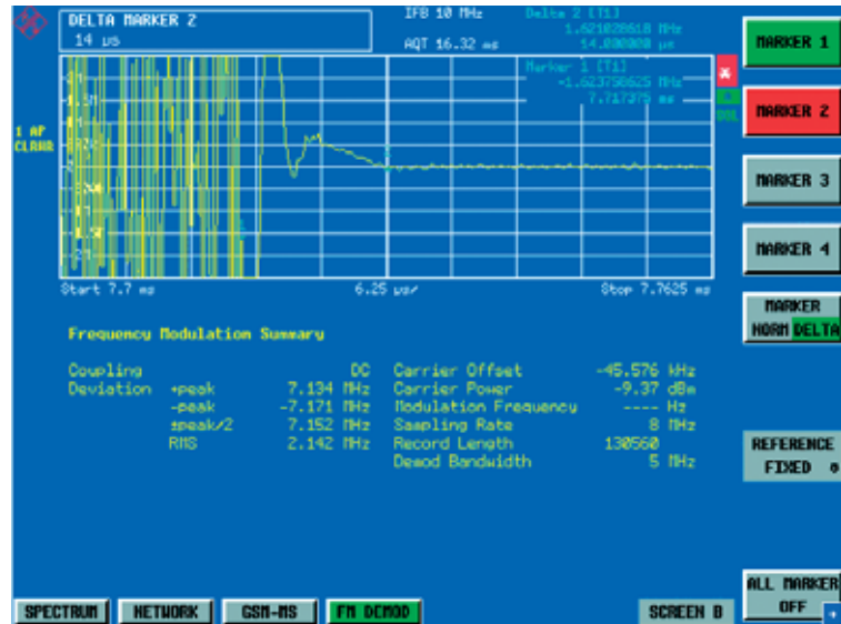
Settling of a synthesizer.
