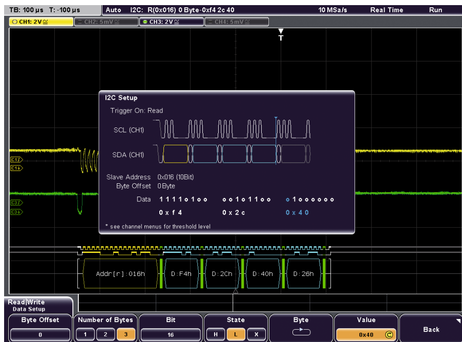
Decoded hexadecimal I 2 C message.
