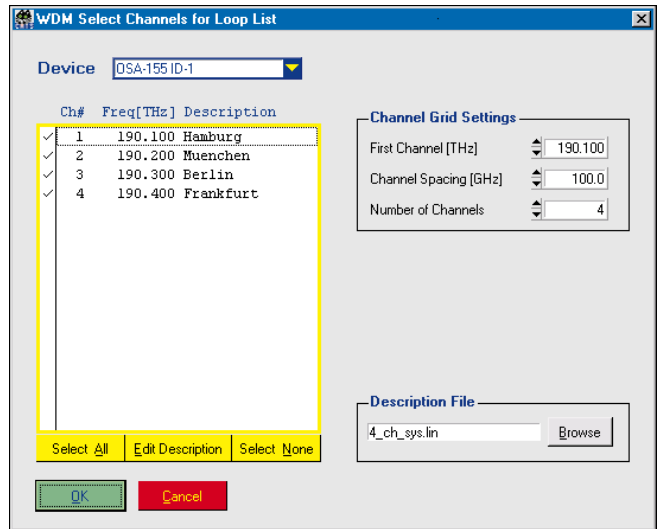
Fully automatic channel selection with CATS DWDM
