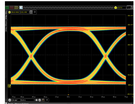
10 Gbps eye captured with 10 GHz of bandwidth.
