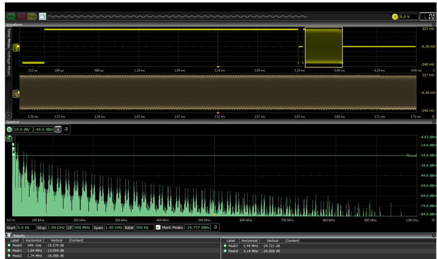
The Z-Series FFT quickly identifies peaks and has key controls such as span, start, stop, etc. that make the oscilloscope behave more like a spectrum analyzer.
