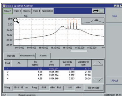
Data acquisition through OSA application.
