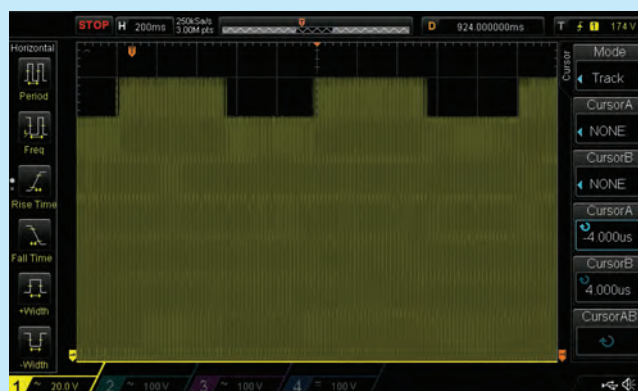
Voltage Modulation Test @ 1Hz Captured
