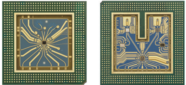
Infiniium's custom multi-chip modules feature indium phosphide chips and Keysight proprietary packaging technology, enabling high bandwidth and low noise.
