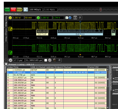
Protocol decode.
