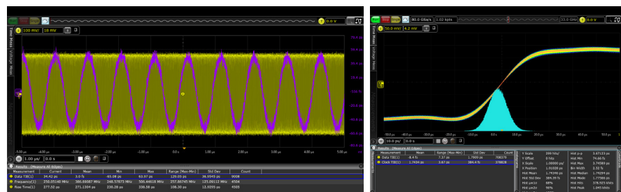
With the 63 GHz bandwidth, the Z-Series is able to effectively characterize the time interval error trend of high speed signals as well as fast rising edges, down to 5 ps.
