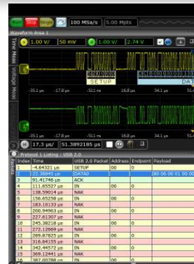
Protocol decode
