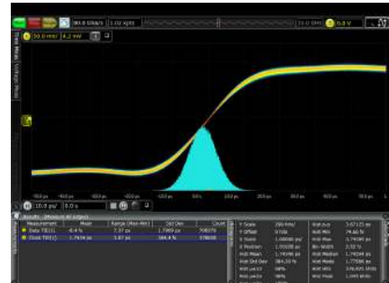
With its flat frequency response and low noise, the Z-Series is able to accurately measure jitter components such as ISI.
