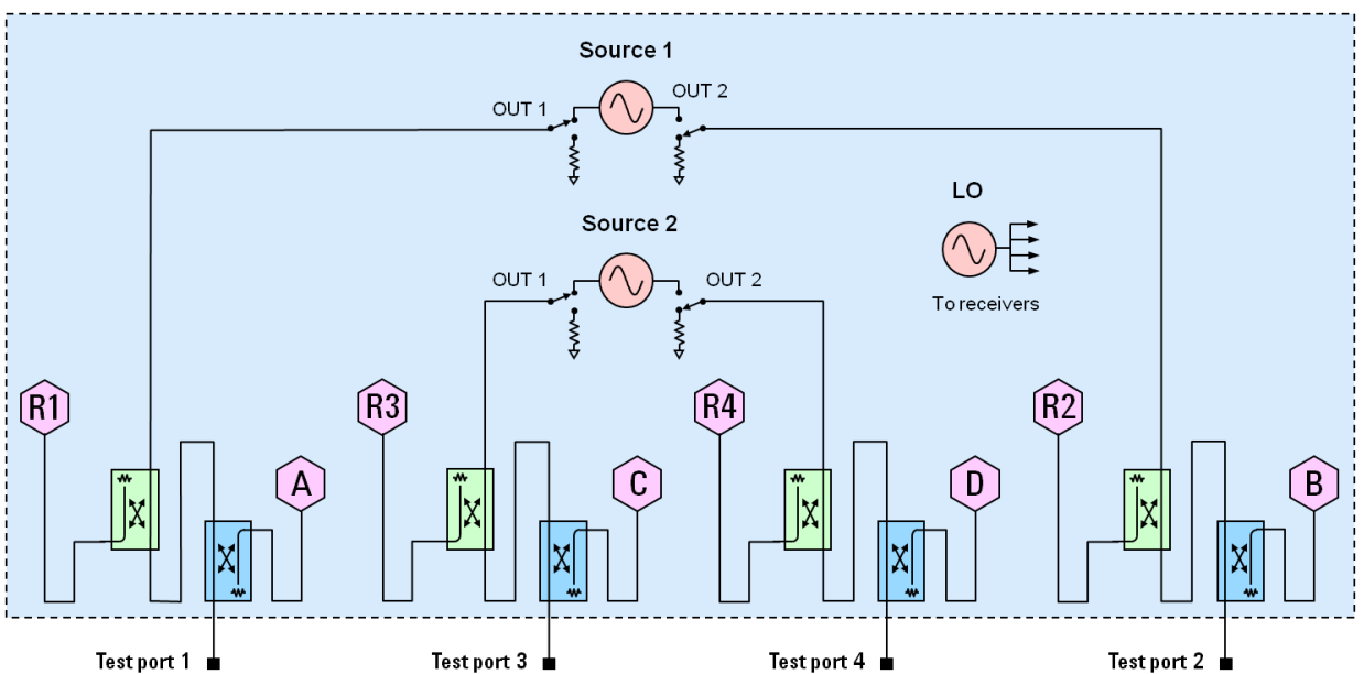
N5224B and N5225B Option 410 (4-port metrology configuration)
