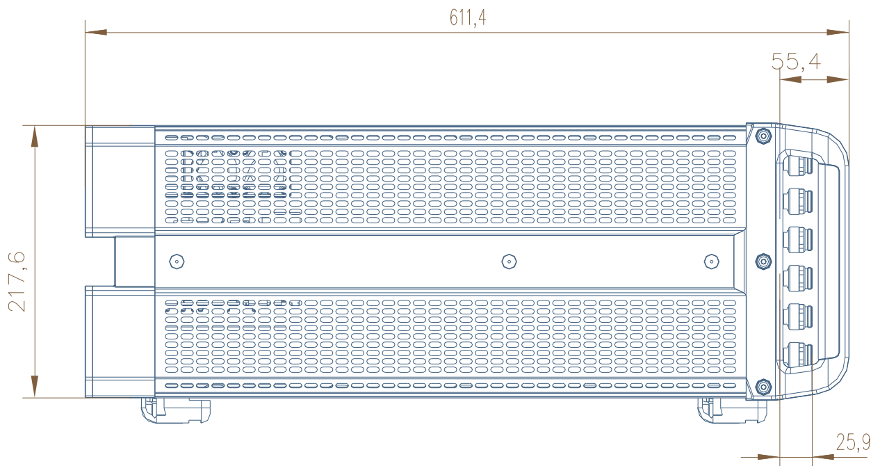
Side view of the R&S®ZNBT20, the R&S®ZNBT26 and the R&S®ZNBT40
