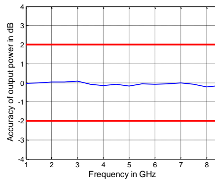
Output power accuracy in dB versus frequency for the R&S ® ZNBT8.
