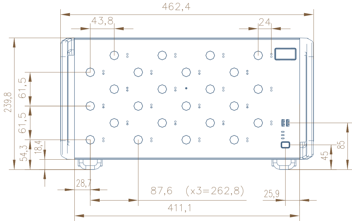
Front view of the R&S®ZNBT8.
