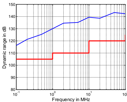
Dynamic range in dB versus frequency for the R&amp;S®ZNBT20.
