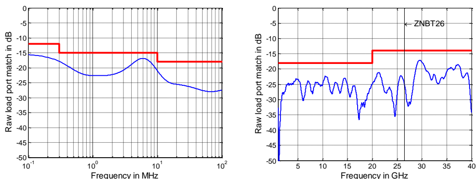
Raw load port match versus frequency for the R&S®ZNBT26/40.
