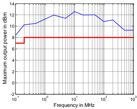
Maximum output power in dBm versus frequency for the R&S ® ZNBT26/40.
