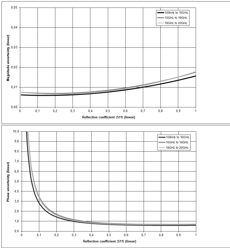
Typical accuracy of reflection magnitude and reflection phase measurements for the R&S® ZNBT20 in the frequency range from 100 kHz to 20 GHz, calibrated with a R&S® ZV-Z235 calibration kit that has been characterized with a DAkkS-accredited calibration. Analysis conditions: S_{12} = S_{21} = 0 , cal. power -10 dBm, meas. power -10 dBm.
