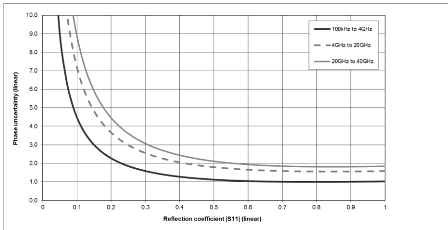
Typical accuracy of reflection magnitude and reflection phase measurements for the R&S® ZNBT40 in the frequency range from 100 kHz to 40 GHz, calibrated with a R&S® ZV-Z235 calibration kit that has been characterized with a DAkkS-accredited calibration. Analysis conditions: S_{12} = S_{21} = 0 , cal. power -10 dBm, meas. power -10 dBm.
